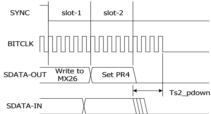
Figure 8. AC-Link Low Power Mode Timing Diagram
