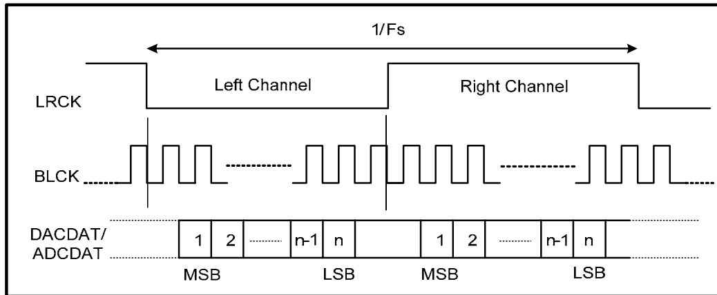
Figure 12. I²S Data Format (bclk_polarity=0)
