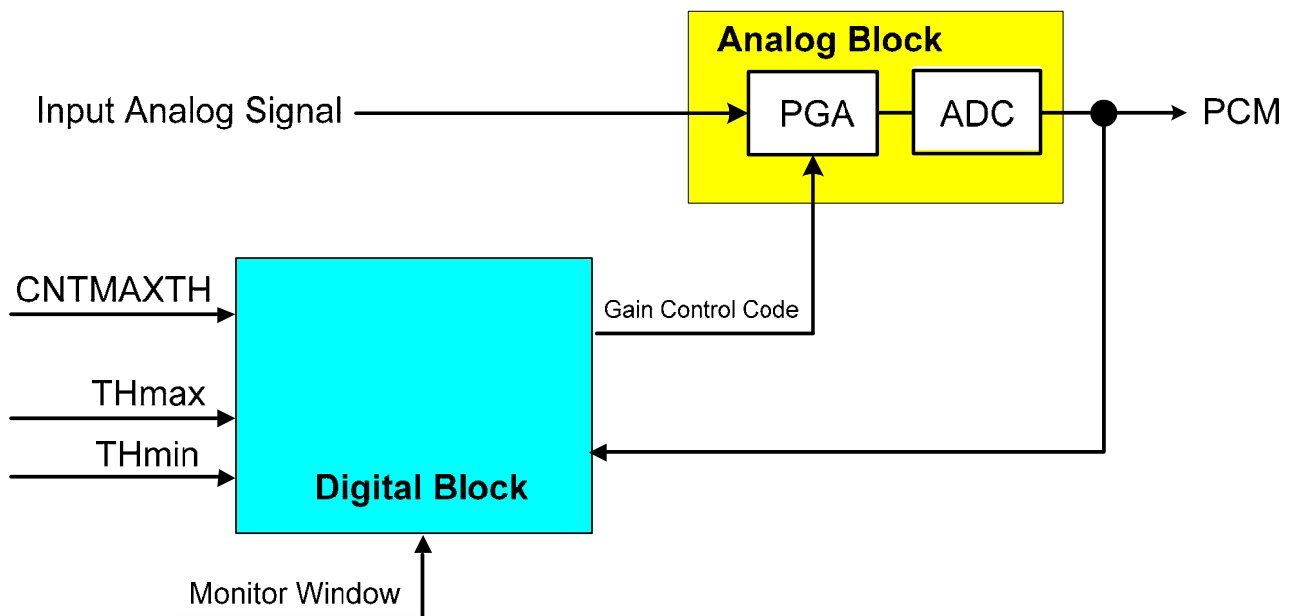
Figure 18. Auto Volume Control Block Diagram
