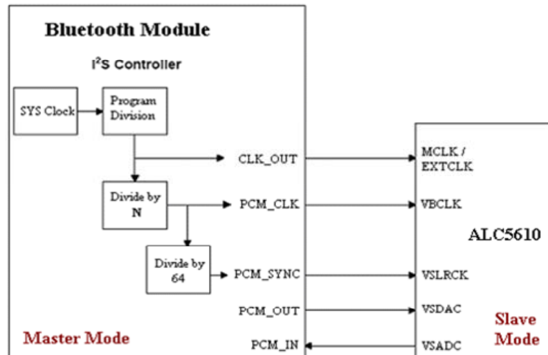
Figure 15. I²S Signal Link Slave Mode Diagram (ALC5610 is Slave)
