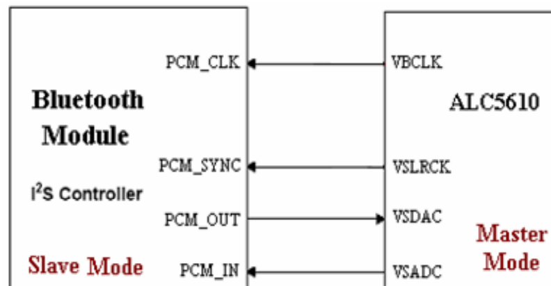
Figure 16. I²S Signal Link Master Mode Diagram (ALC5610 is Master)
