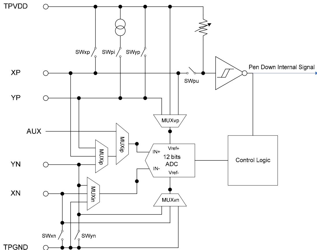
Figure 17. 4-Wire Resistive Touch Panel Circuit
