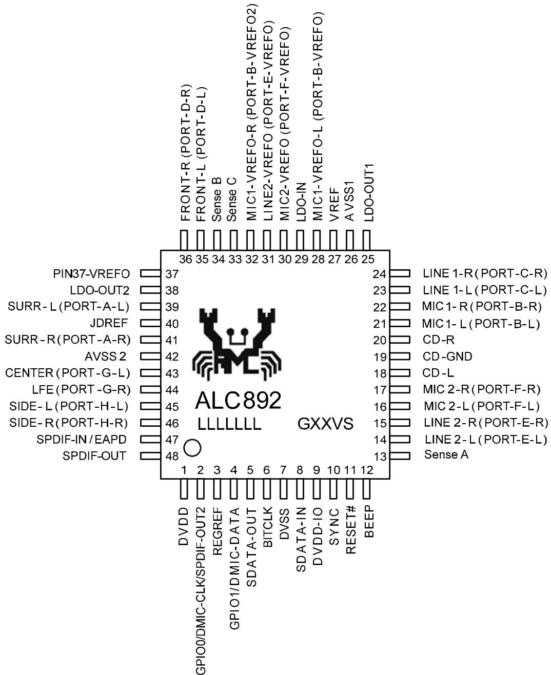
Figure 3. Pin Assignments
