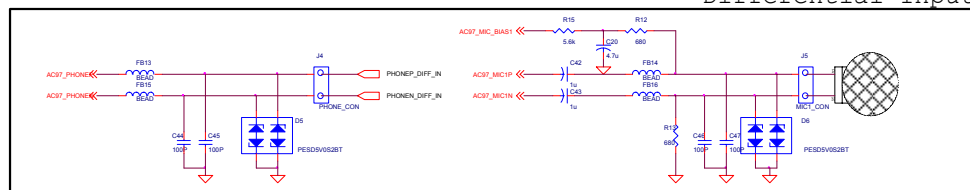
Differential Input
