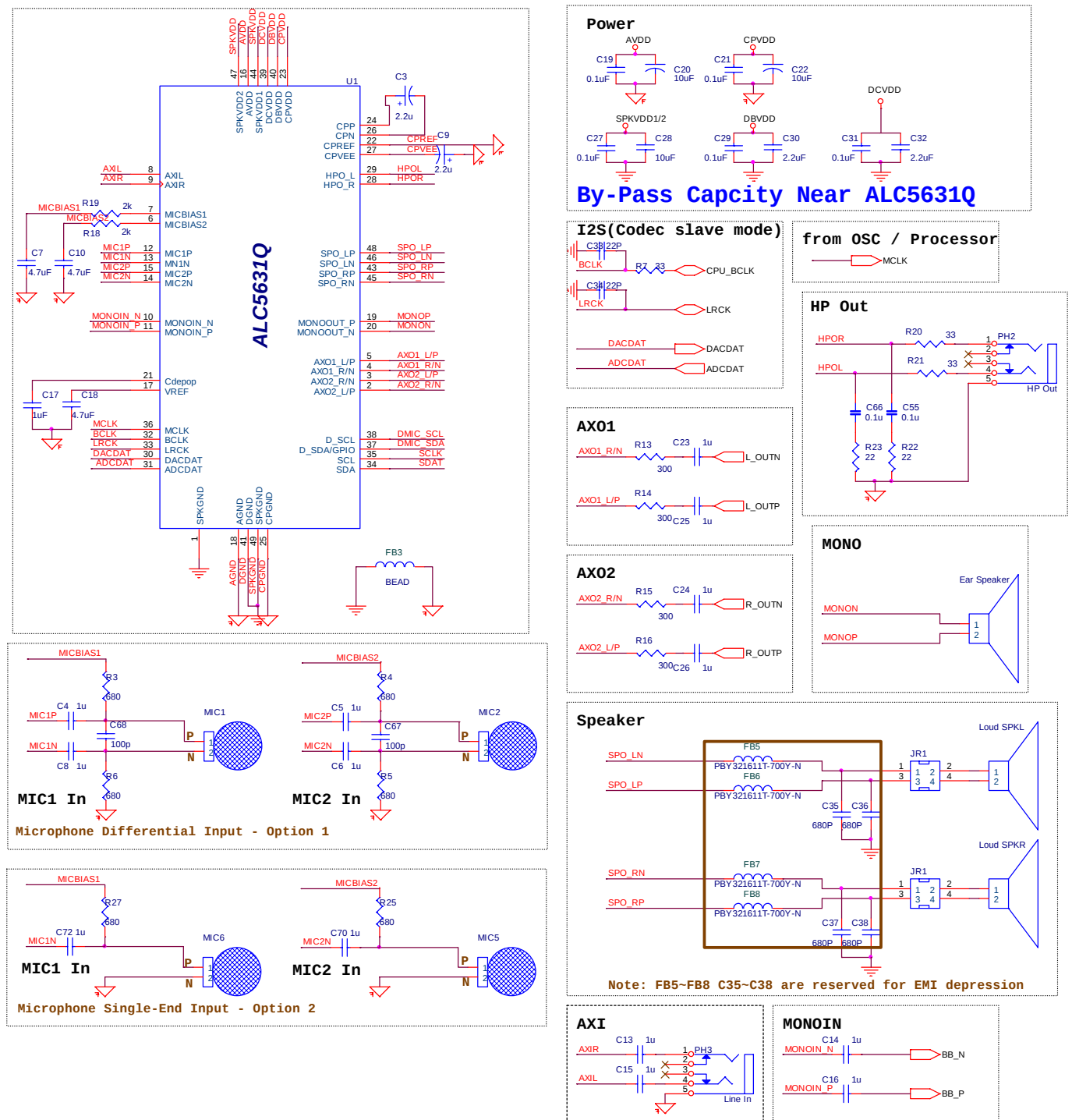
Figure 21. Application Circuit
