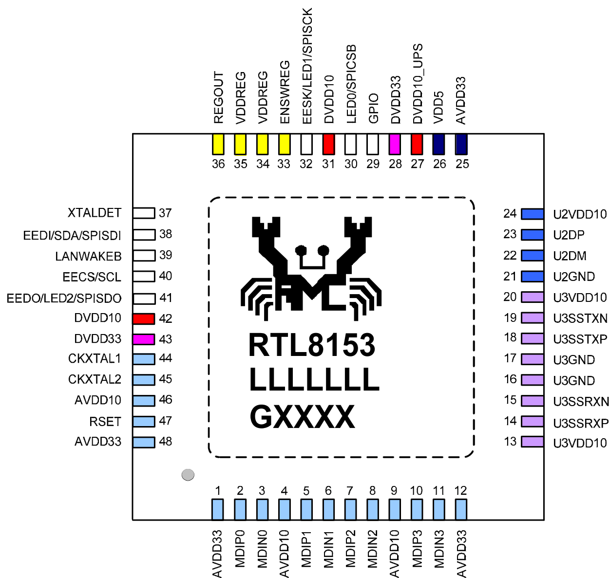
Figure 1. Pin Assignments
