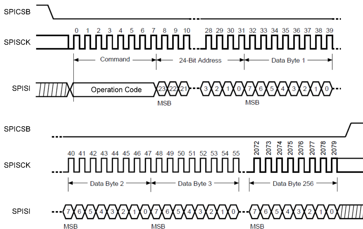
Figure 9. Page Program Timing Sequence
