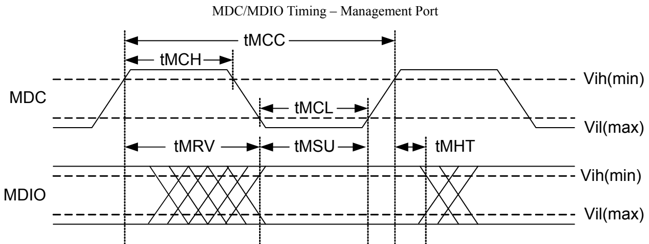
Figure 18. MDC/MDIO Management Timing Parameters
