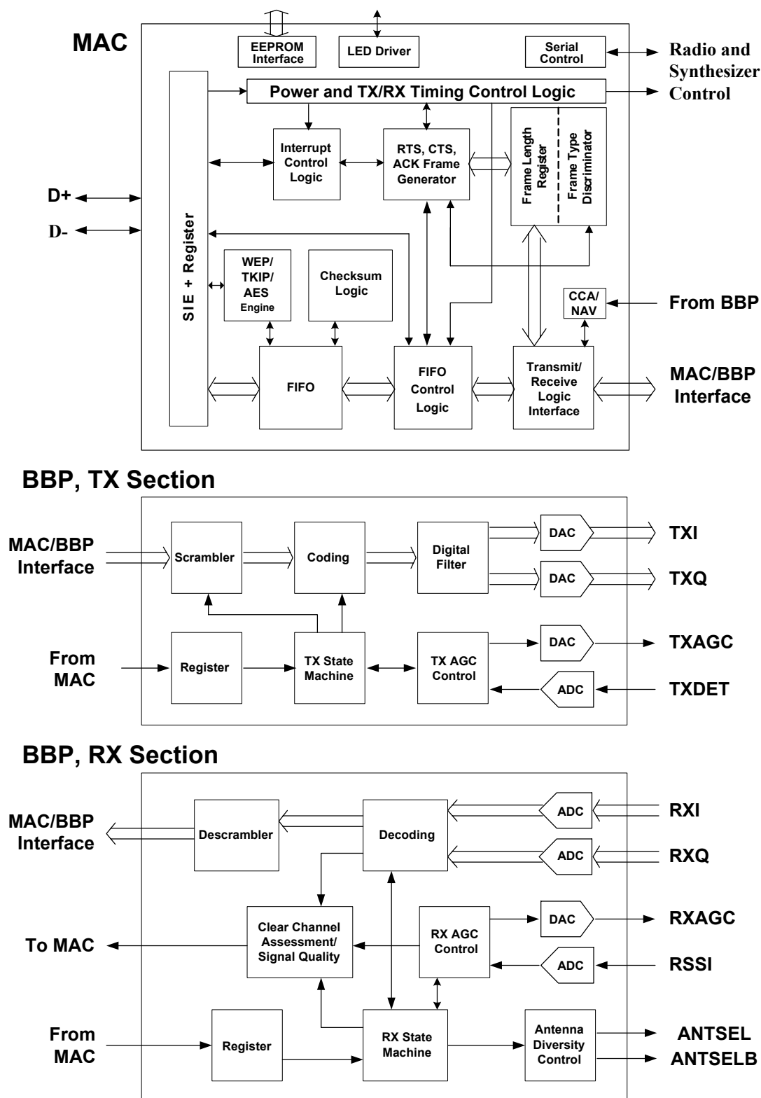
Figure 1. Block Diagram
