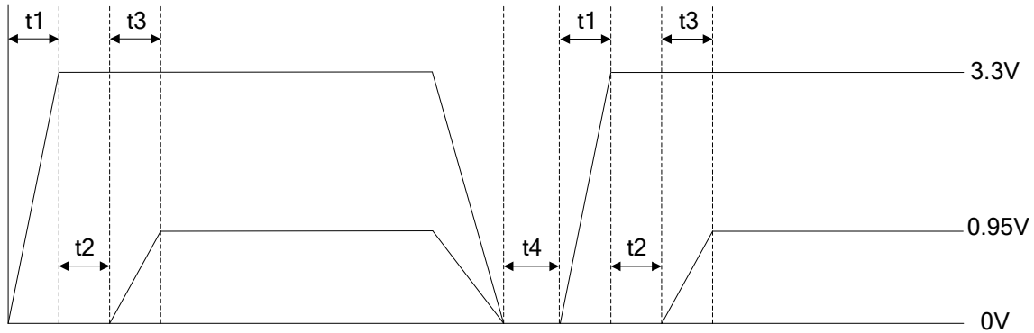
Figure 6. Power Sequence
