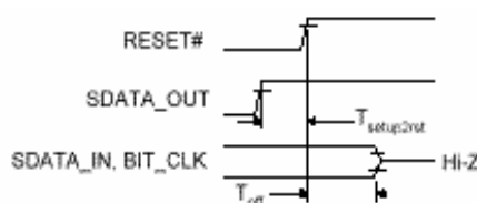
ATE test mode timing diagram
