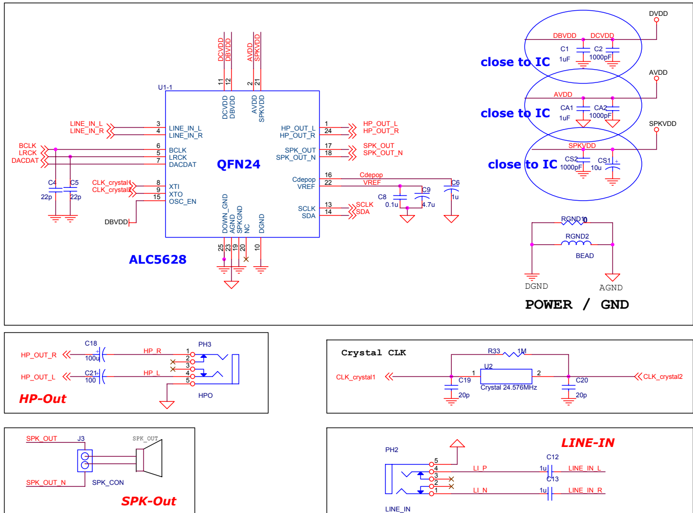
Figure 20. Application Circuits
