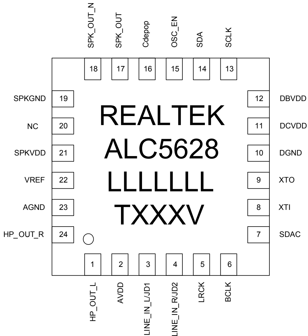
Figure 3. Pin Assignments
