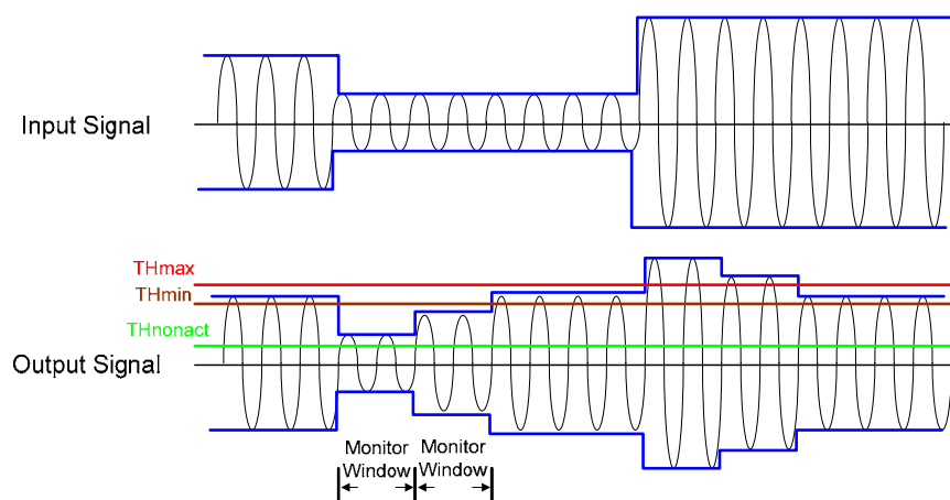
Figure 13. AVC Behavior
