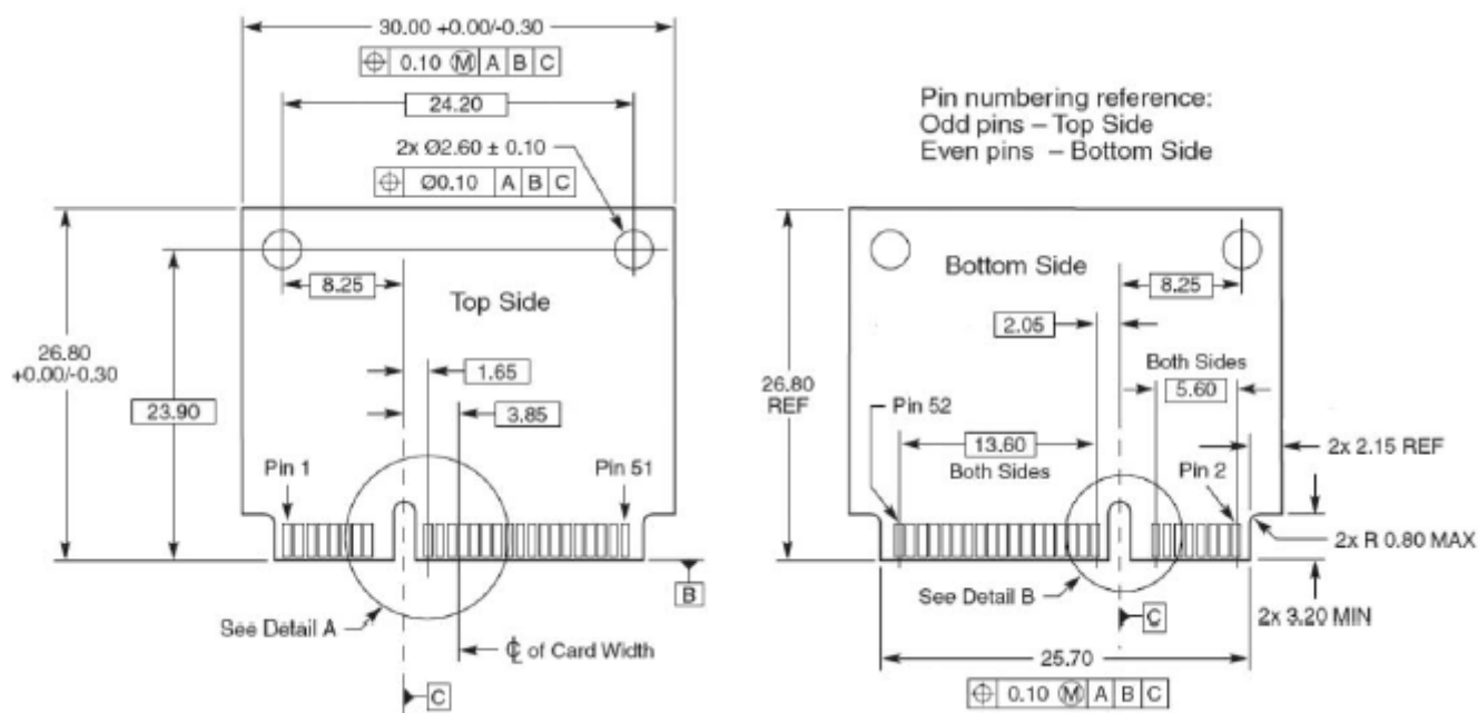
Figure 1. RTL8192DE Half Mini-Card Mechanical Specification
