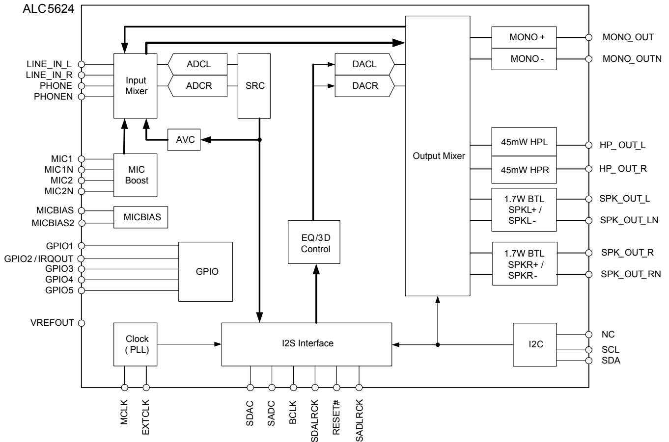
Figure 1. Block Diagram
