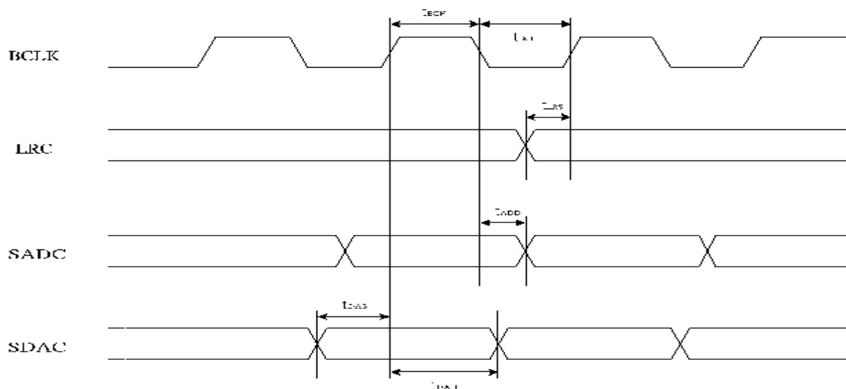
Figure 17. I 2 S/PCM Slave Mode Timing
