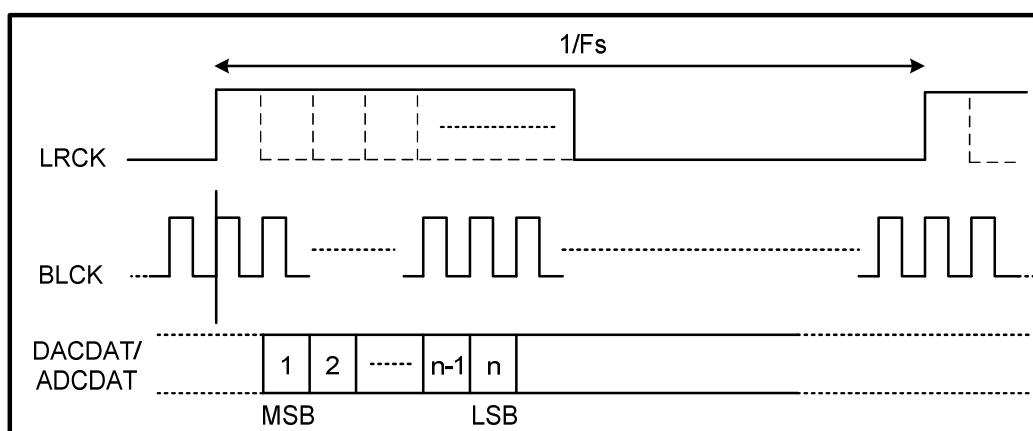
Figure 5. PCM MONO Data Mode A Format (BCLK POLARITY=1)
