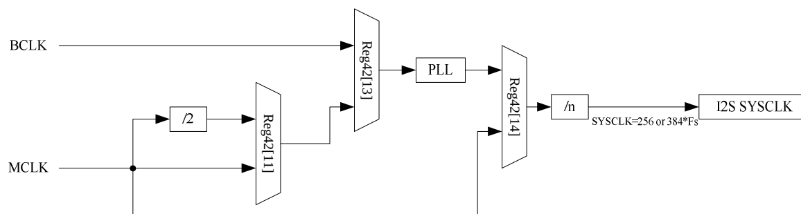
Figure 4. Audio Clock
