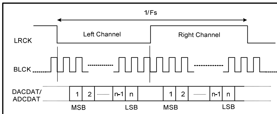
Figure 9. I²S Data Format (BCLK POLARITY=0)
