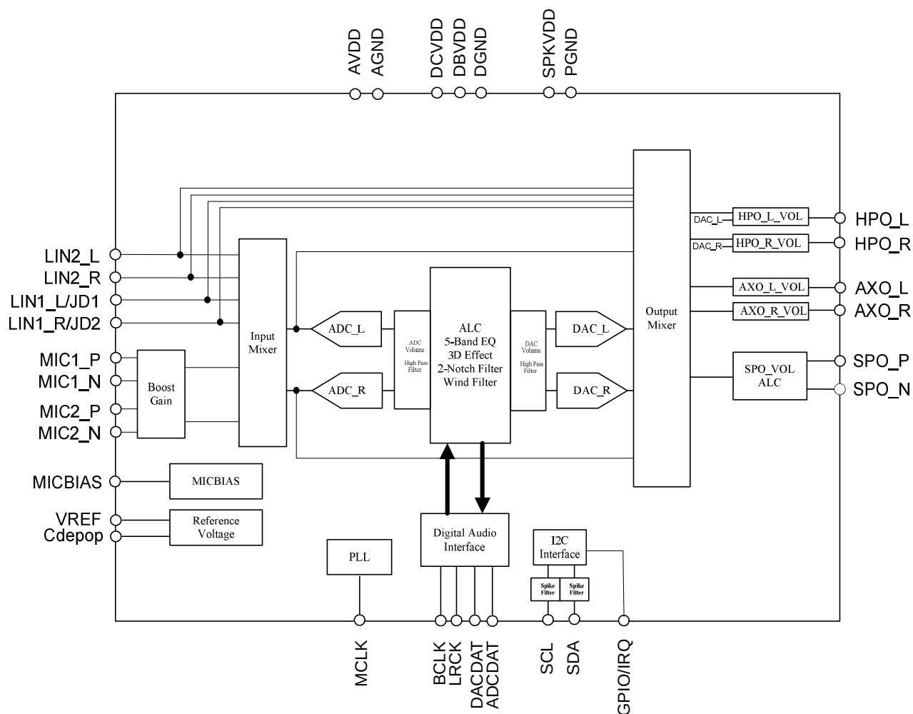
Figure 1. Block Diagram
