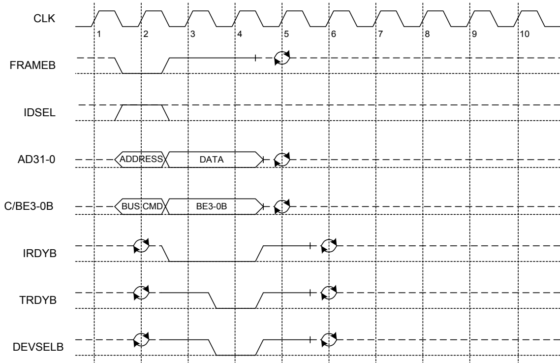
Figure 15. Configuration Write
