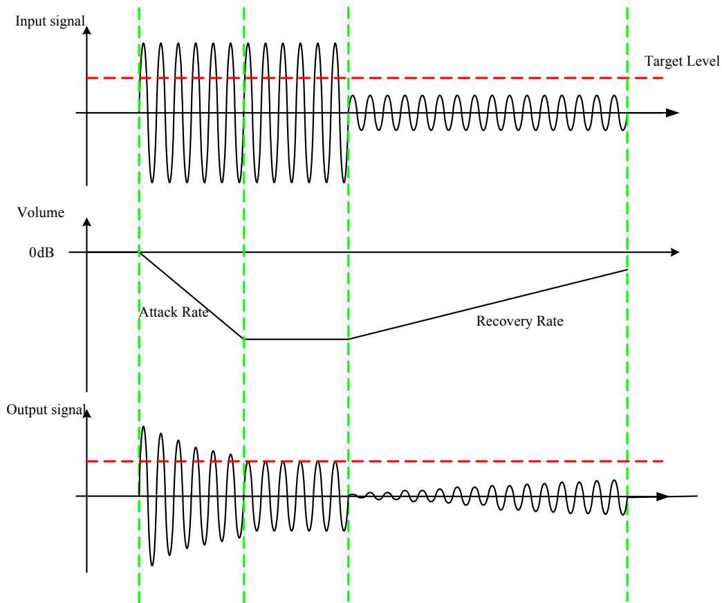
Figure 18. DRC/AGC for Playback/Recording Mode
