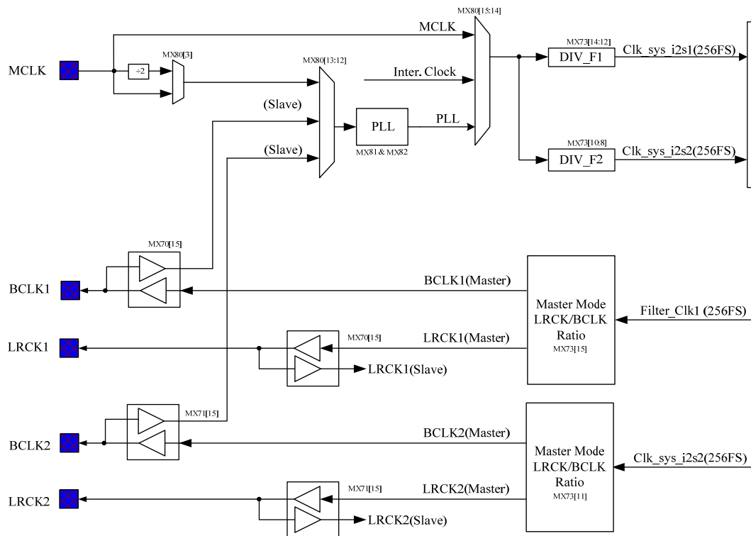
Figure 5. Audio Clock Tree
