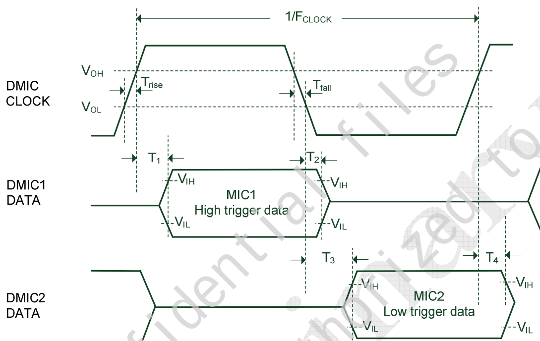
Figure 29. Audio Digital Microphone Timing Diagram
