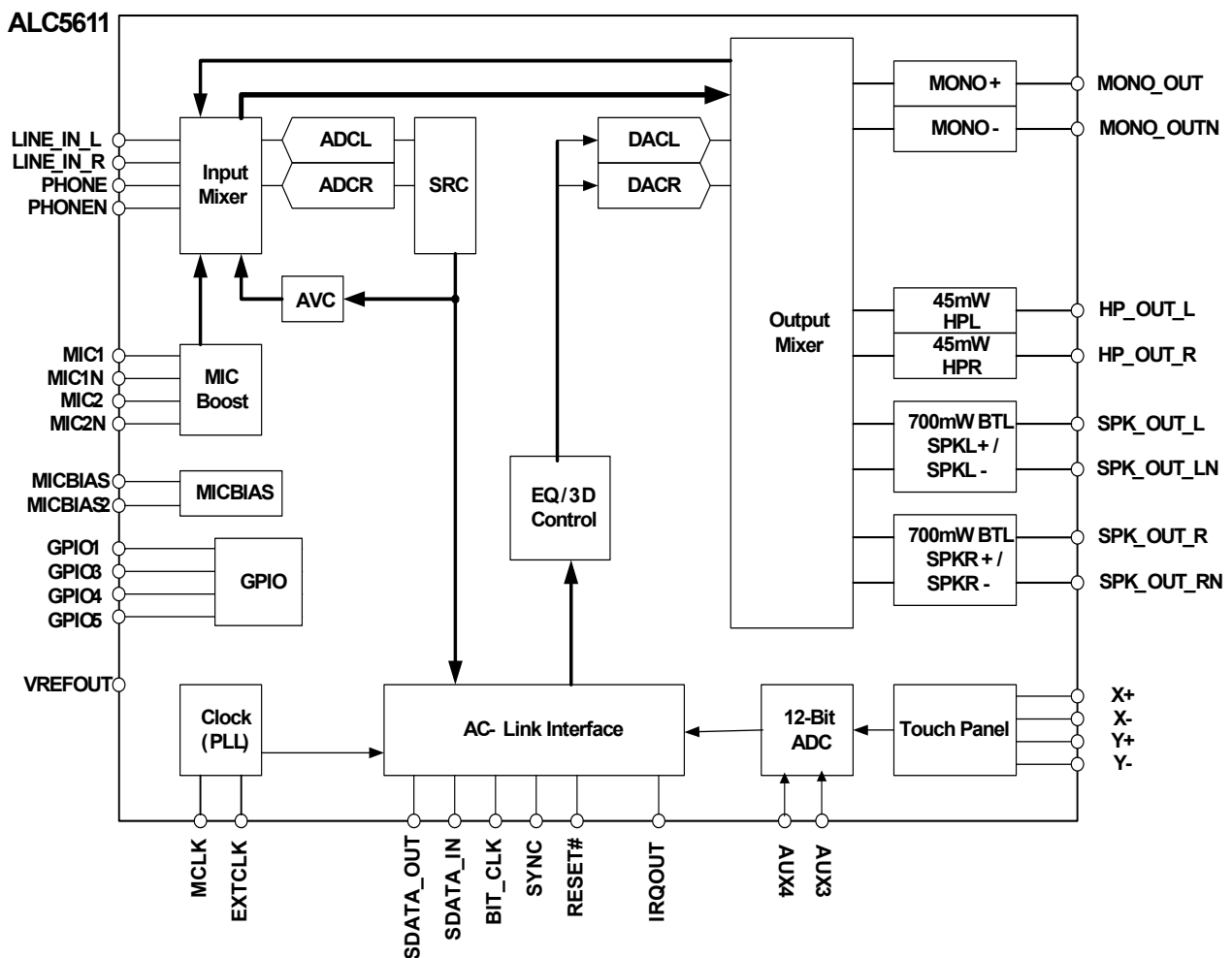
Figure 1. Block Diagram
