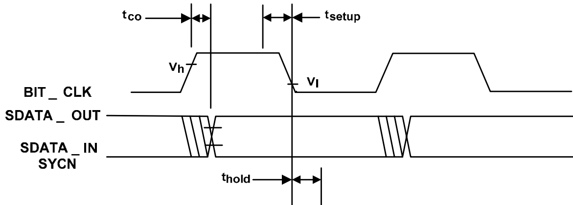
Figure 16. Data Output and Input Timing
