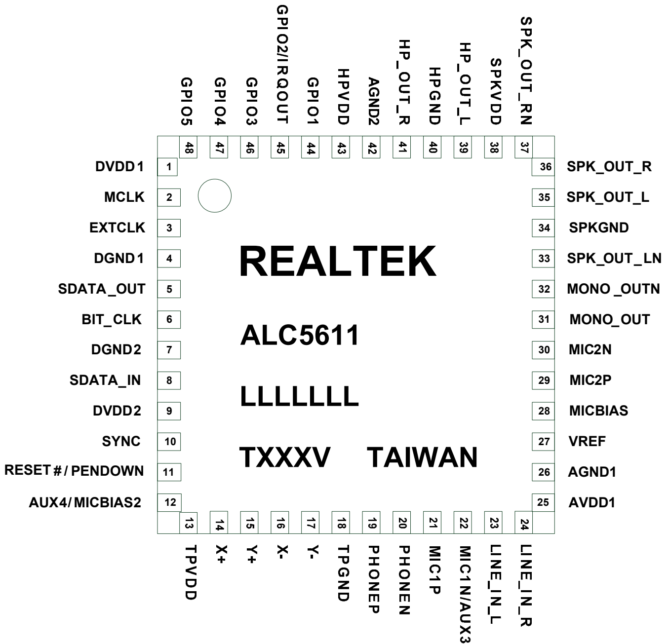
Figure 3. Pin Assignments
