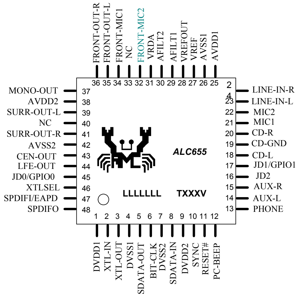
Figure 1. Pin Assignments
