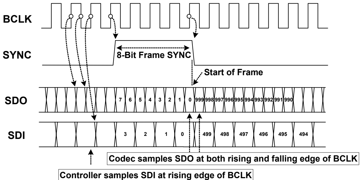
Figure 6. Bit Timing
