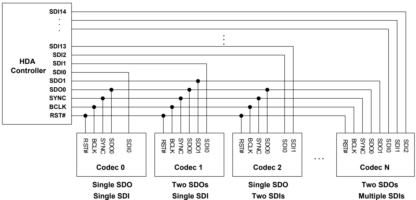
Figure 7. Signaling Topology
