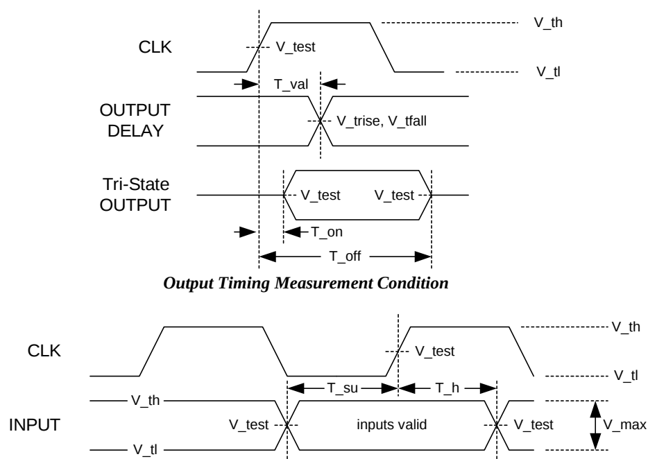
Input Timing Measurement Conditions
