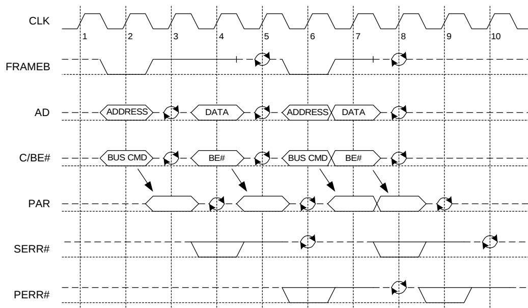
Parity Operation - One Example
