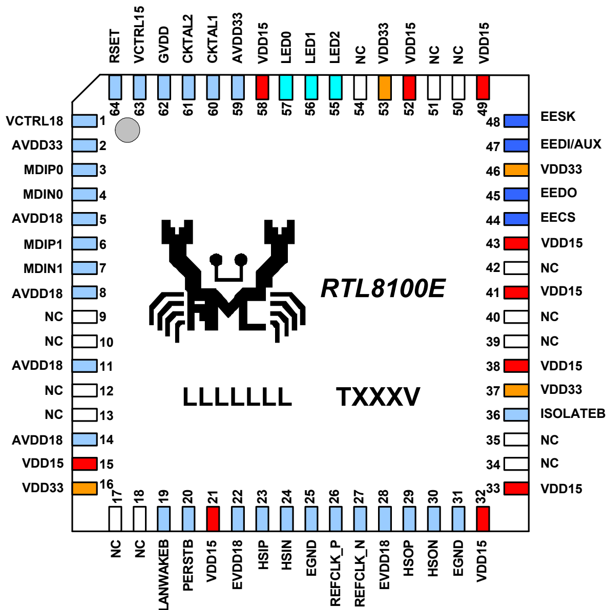
Figure 1. Pin Assignments
