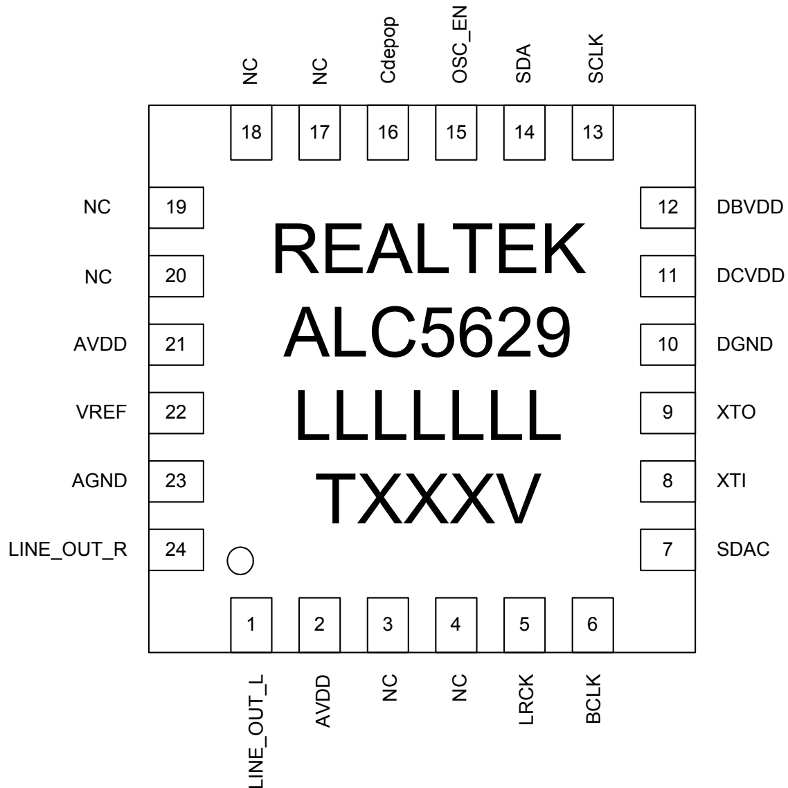
Figure 3. Pin Assignments
