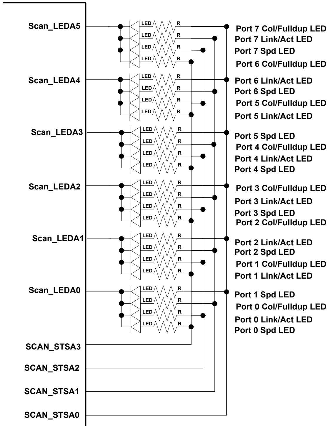
Figure 14. External Circuit for Scan LED
