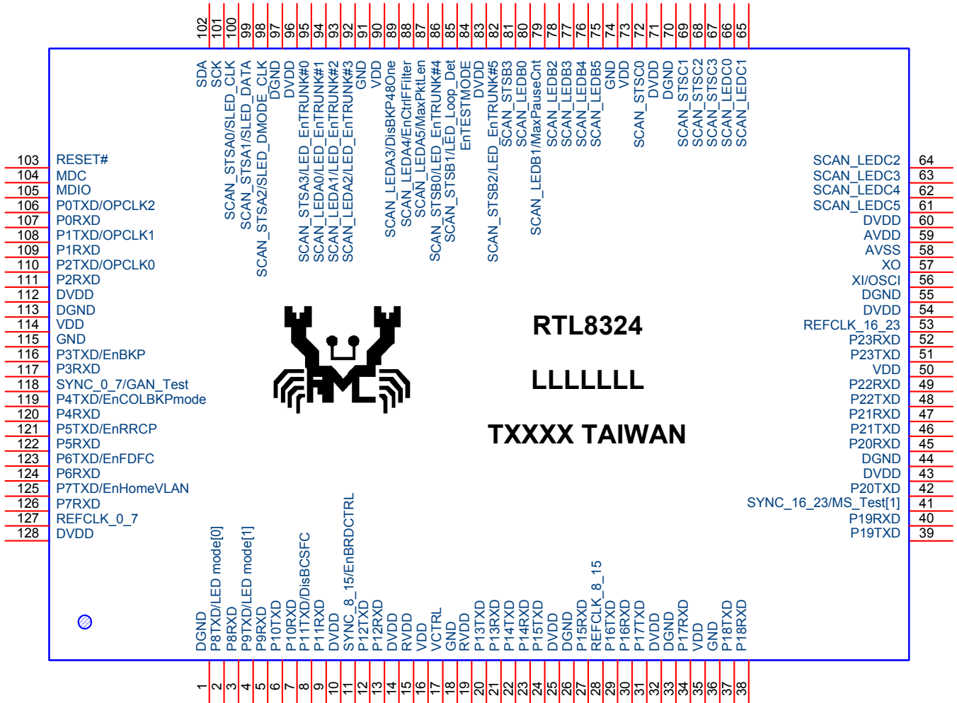
Figure 3. Pin Assignments
