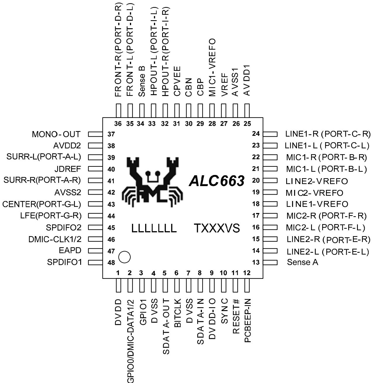
Figure 2. Pin Assignments
