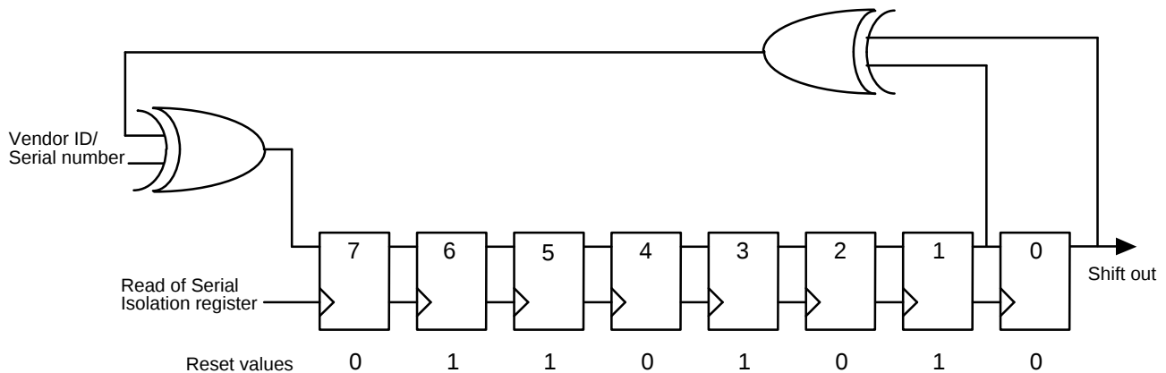
Figure 3. Checksum LFSR
