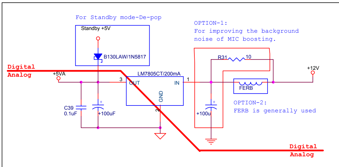
Figure 18. Filter Connection
