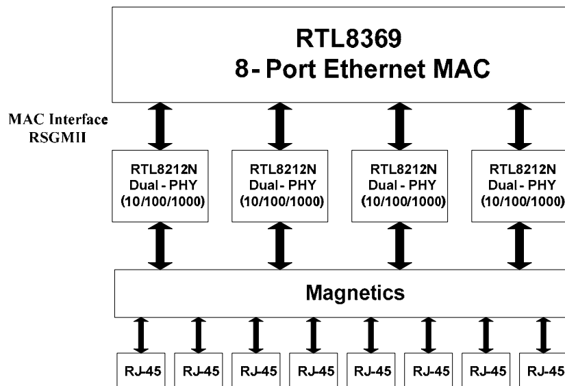
Figure 1. RTL8212N with 8-Port Gigabit MAC (RTL8369)
