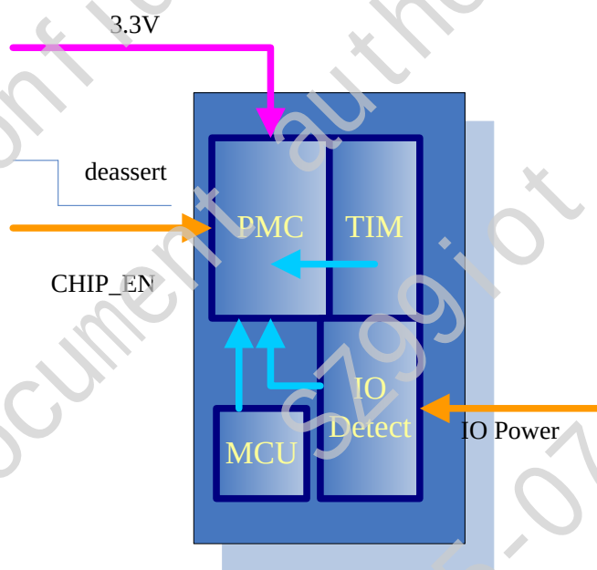
Figure 7 Shutdown Mode
