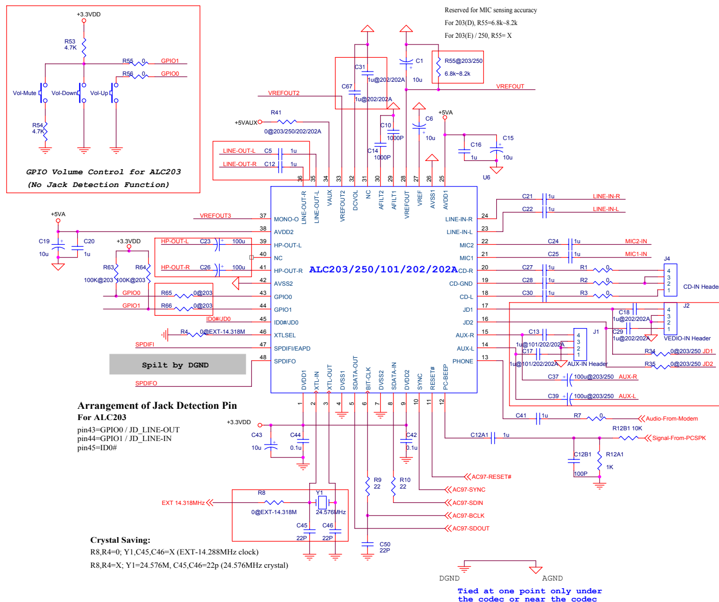
Filter Connection Schematic
