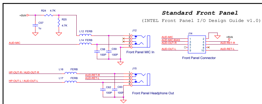
Onboard Header and Reference Front Panel I/O Schematic
