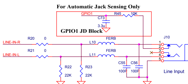
I/O Connection Schematic
