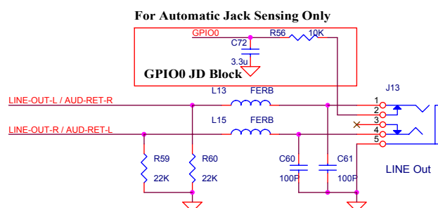
I/O Connection Schematic
