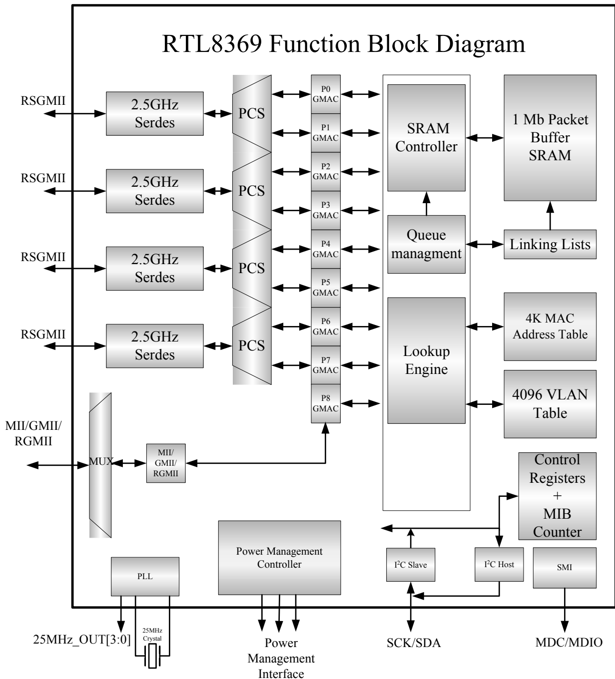
Figure 2. Block Diagram of RTL8369
