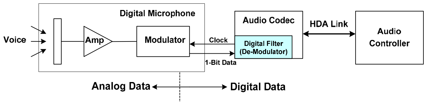
Figure 25. Digital Microphone Implementation-1
