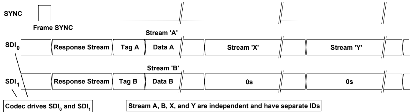
Figure 16. Codec Transmits Data Over Multiple SDIs
