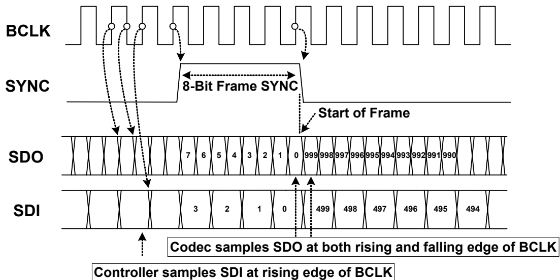
Figure 9. Bit Timing
