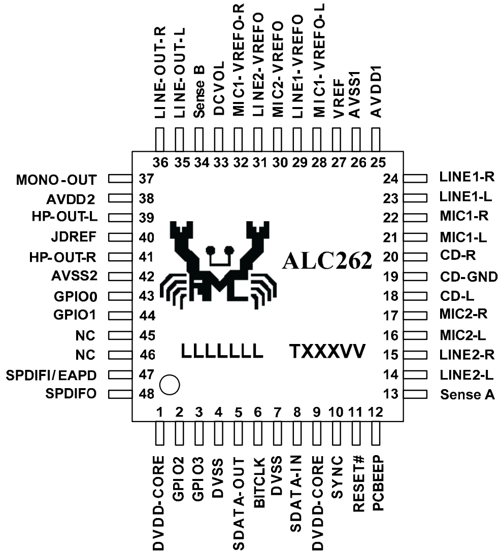
Figure 5. ALC262 A/B Version Pin Assignments
