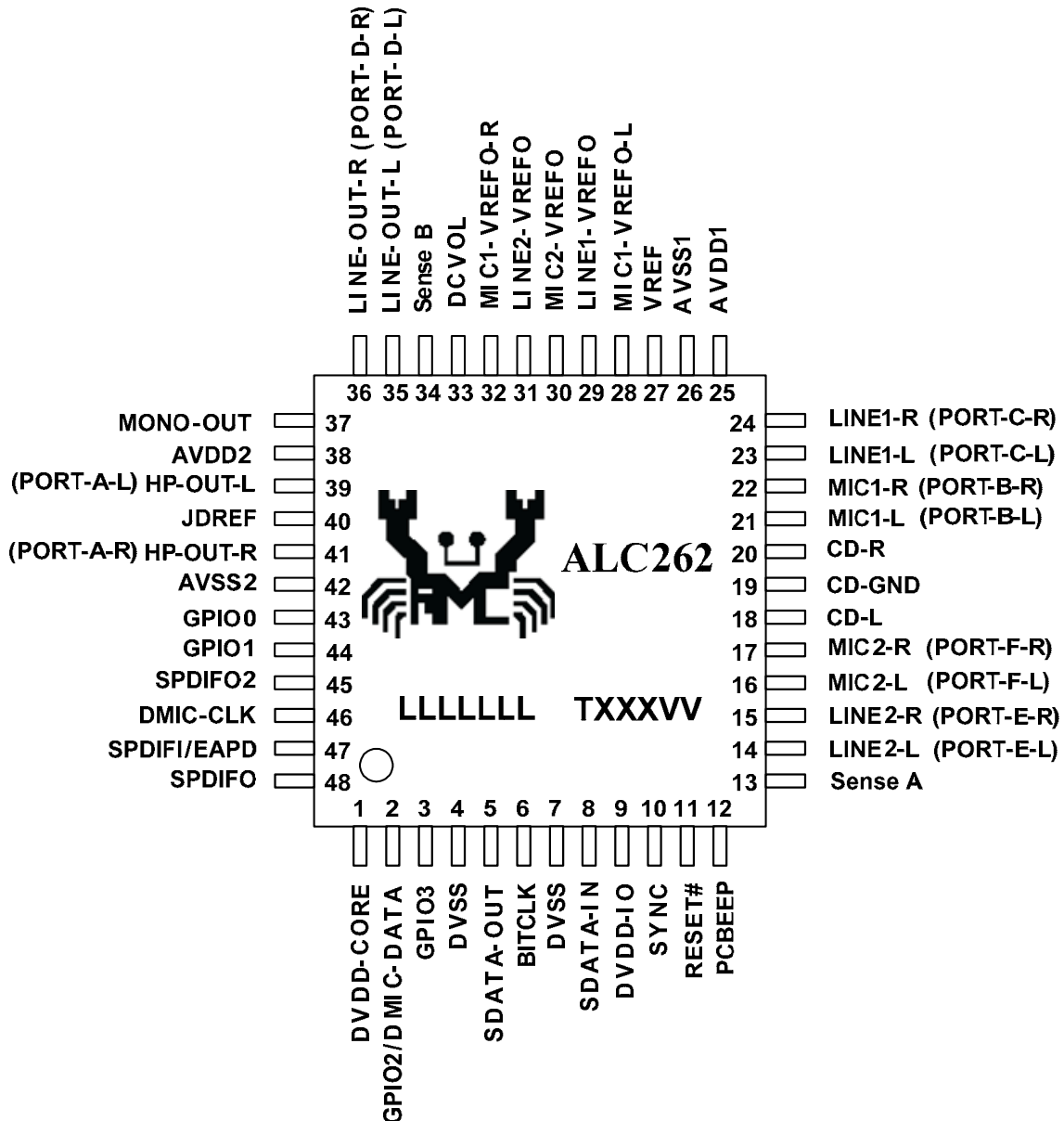
Figure 7. ALC262 D Version Pin Assignments
