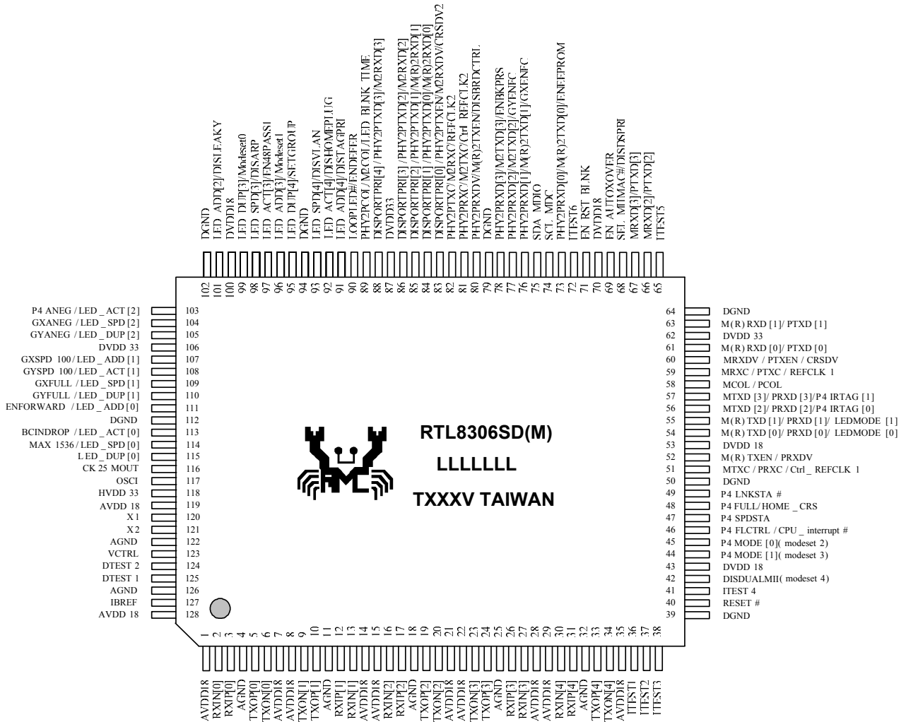
Figure 2. Pin Assignments
