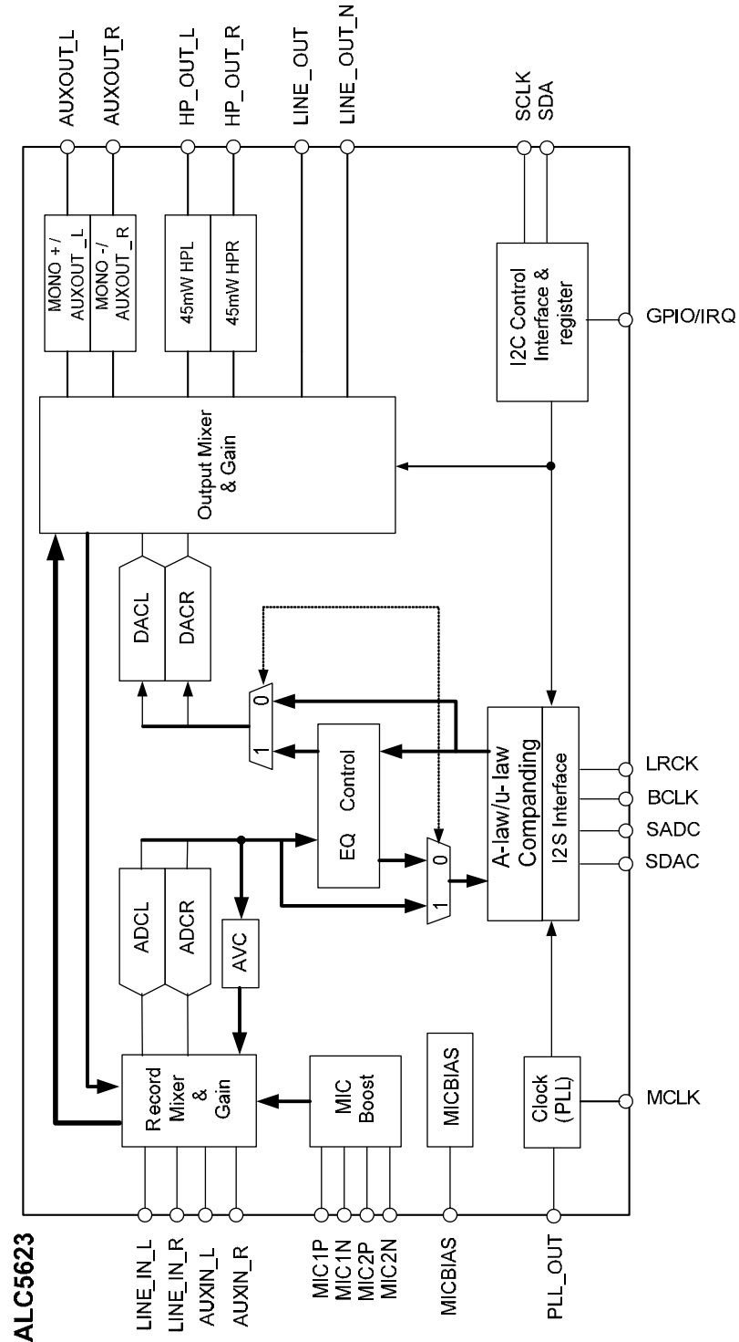
Figure 1. Block Diagram
