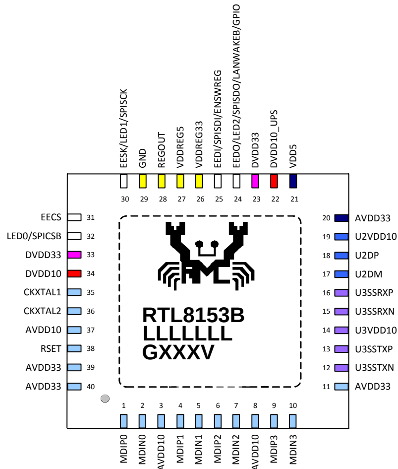
Figure 1. Pin Assignments
