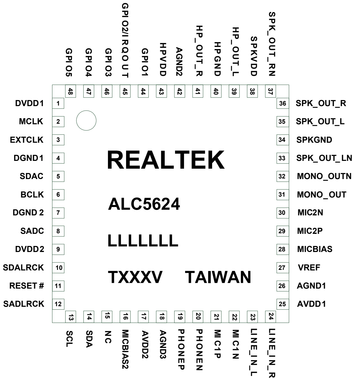
Figure 3. Pin Assignments
