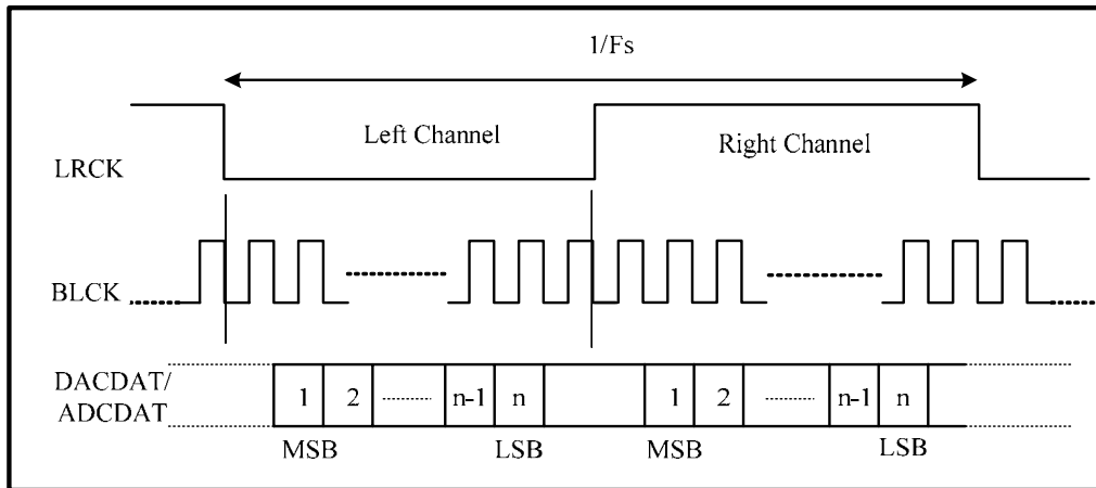
Figure 9. I²S Data Format (bclk_polarity=0)
