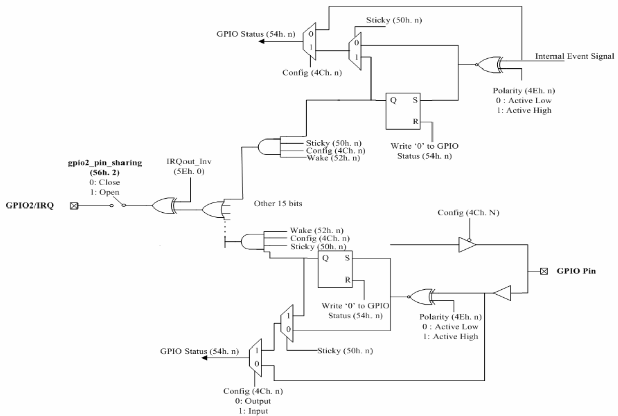
Figure 14. GPIO Implementation
