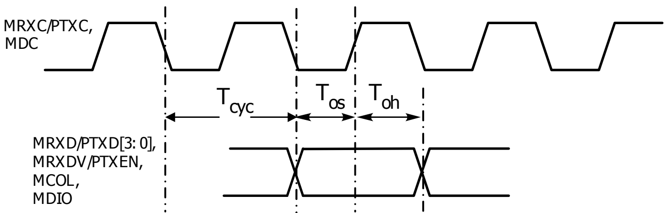
Figure 22. MII Interface Transmission Data Timing
