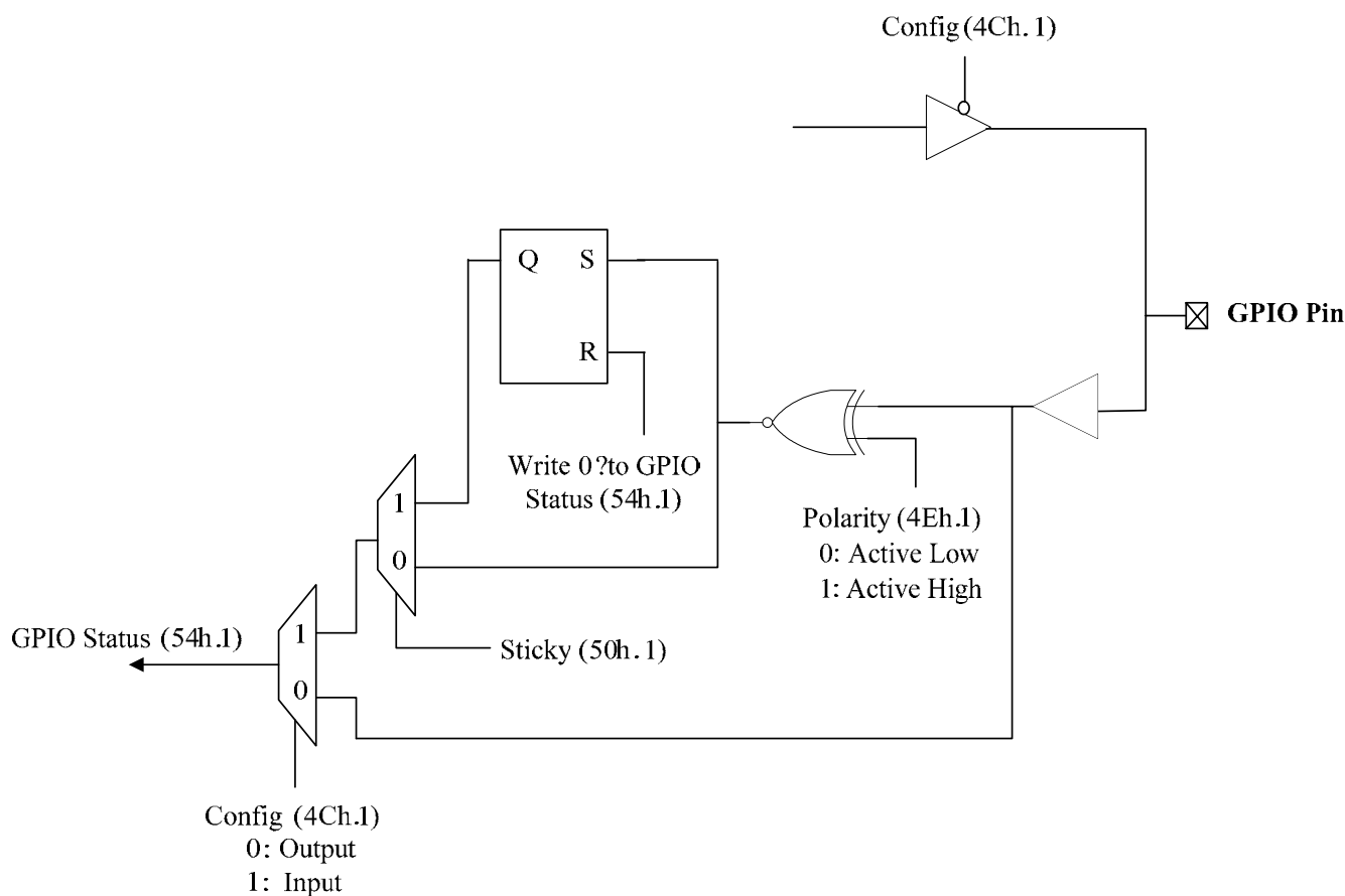
Figure 18. GPIO Implementation
