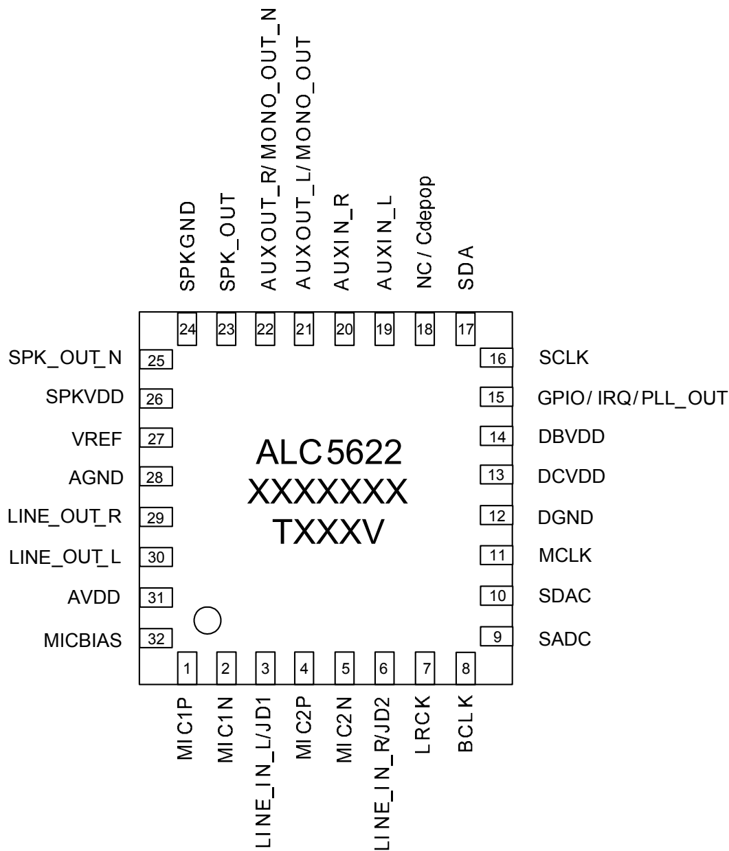
Figure 3. Pin Assignments
