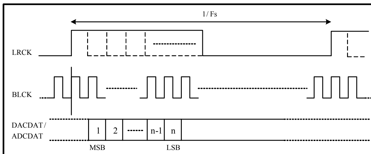
Figure 6. PCM Mono Data Mode A Format (stereo_i2s_bclk_polarity_ctrl=1, pcm_mode_sel=0)
