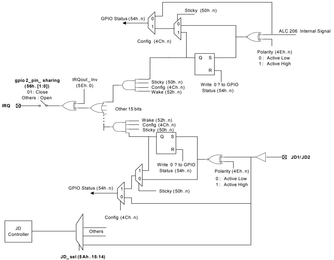
Figure 19. Jack Detect and IRQ Logic
