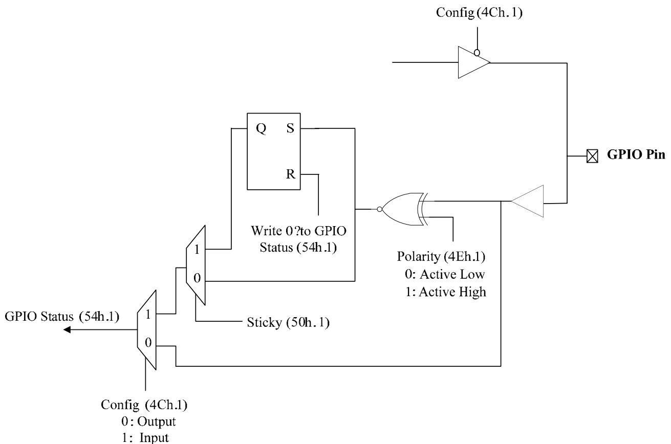
Figure 18. GPIO Implementation
