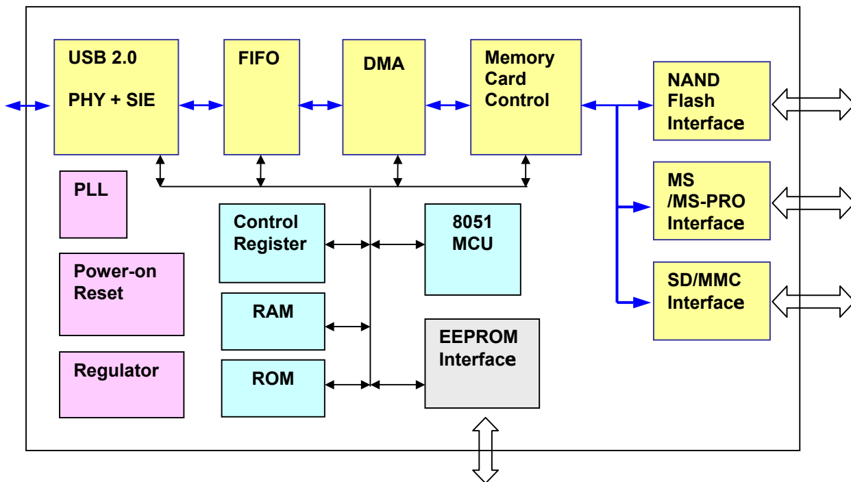
Figure 1. Block Diagram
