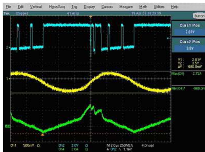
Figure 10. Ceramic 22μF 0805(Y5V) (Bad)
