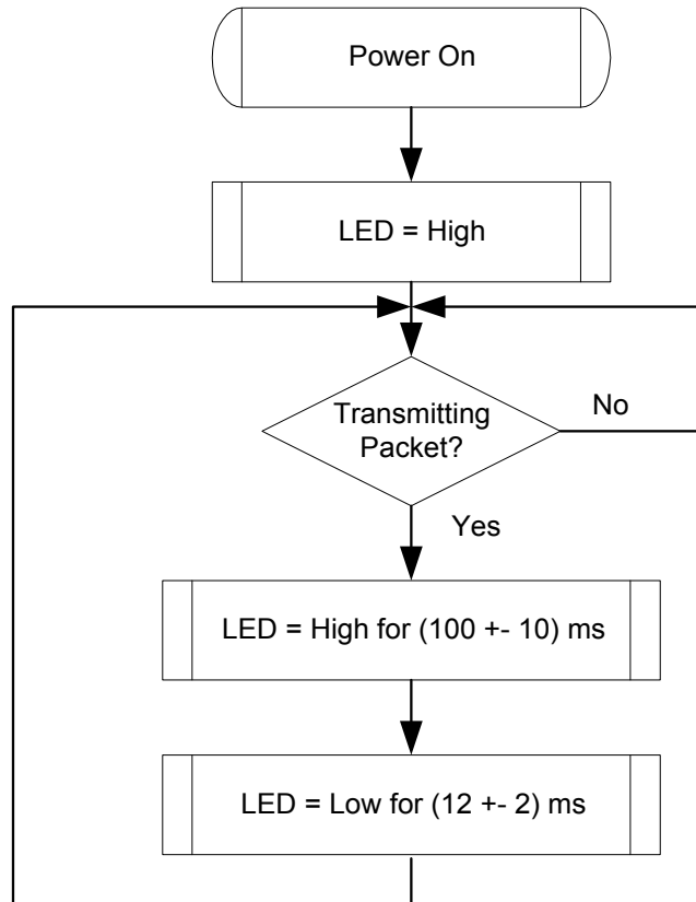
Figure 9. Tx LED
