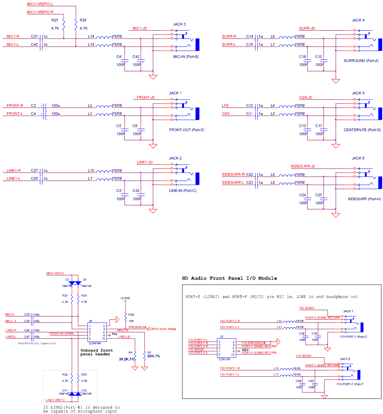
Figure 19. IO Connection
