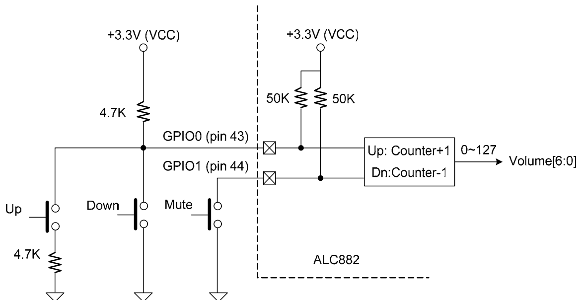
Figure 22. Volume Control by GPIO0 and GPIO1
