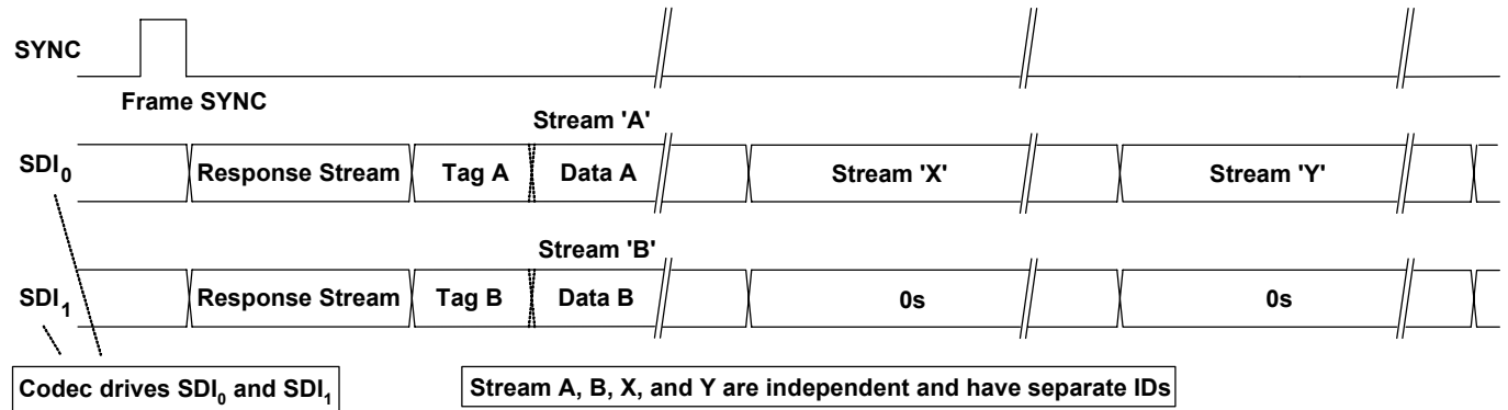
Figure 12. Codec Transmits Data Over Multiple SDI
