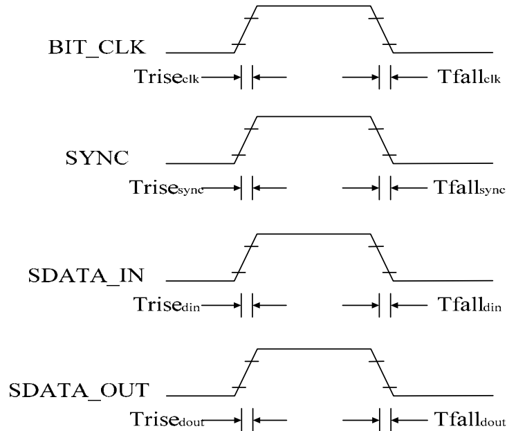
Figure 27. Signal Rise and Fall Timing
