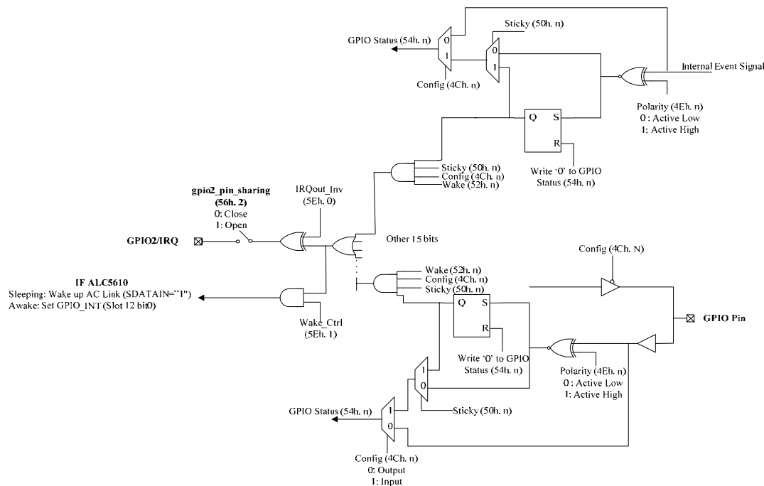
Figure 20. GPIO Implementation
