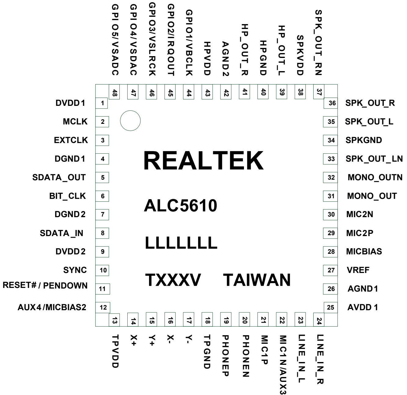
Figure 3. Pin Assignments
