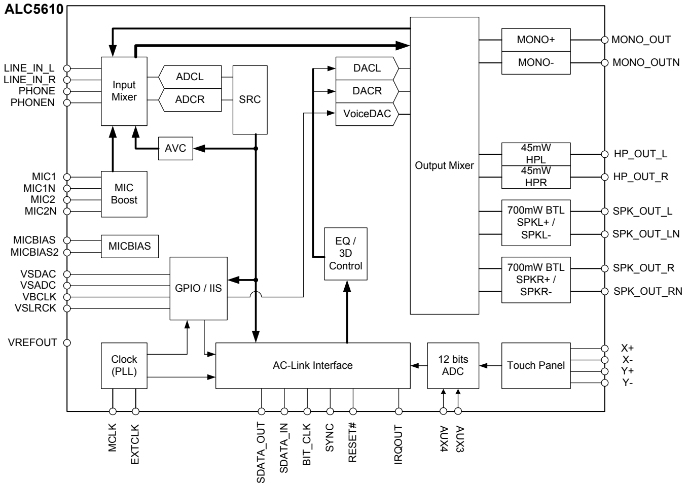
Figure 1. Block Diagram
