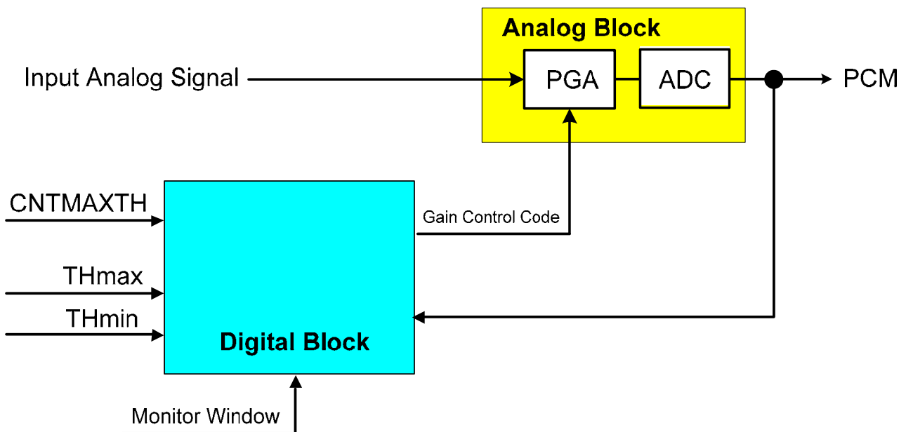
Figure 18. Auto Volume Control Block Diagram
