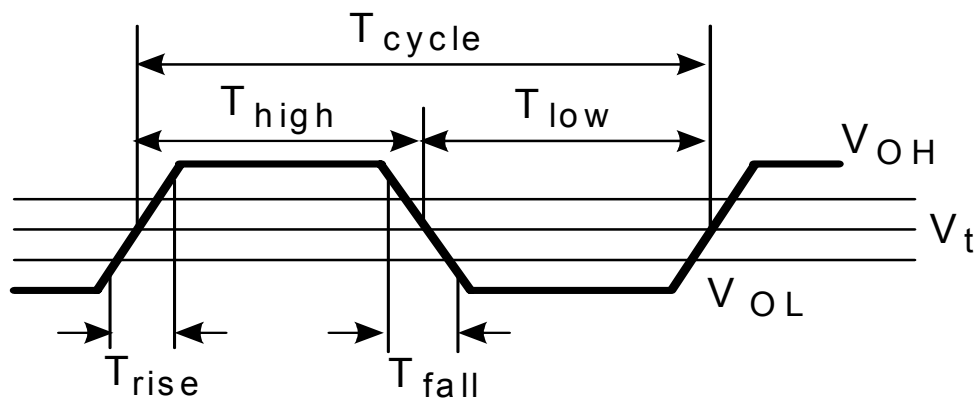
Figure 17. Output Timing
