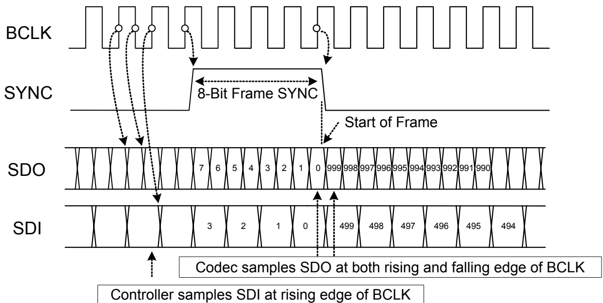
Figure 4. Bit Timing
