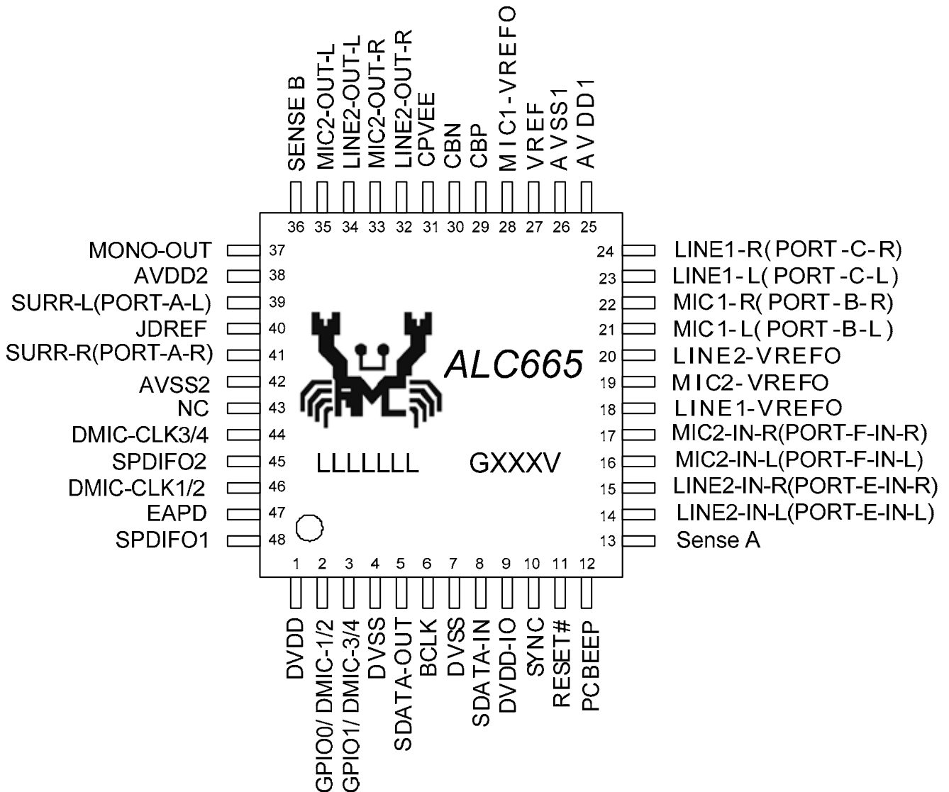
Figure 2. Pin Assignments
