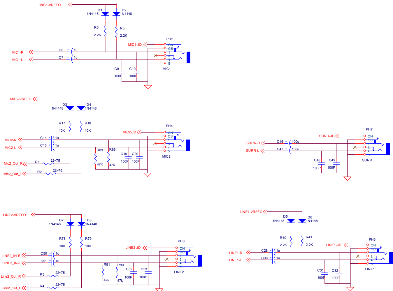
Figure 19. Analog Input/Output Connection
