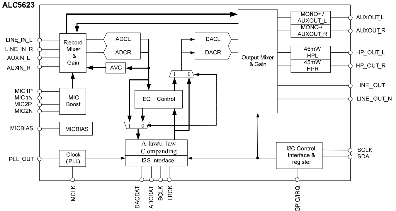
Figure 1. Block Diagram
