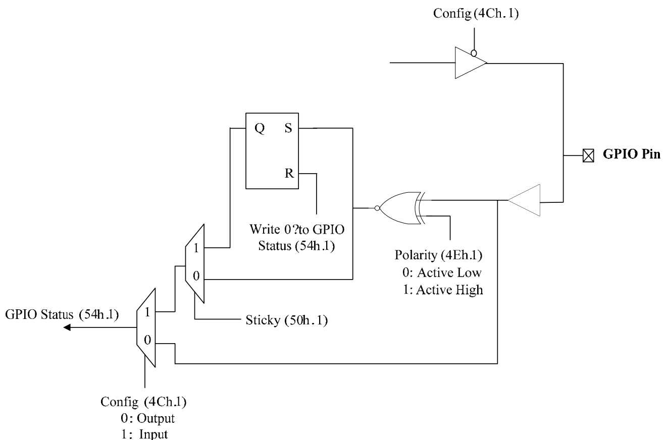
Figure 18. GPIO Implementation
