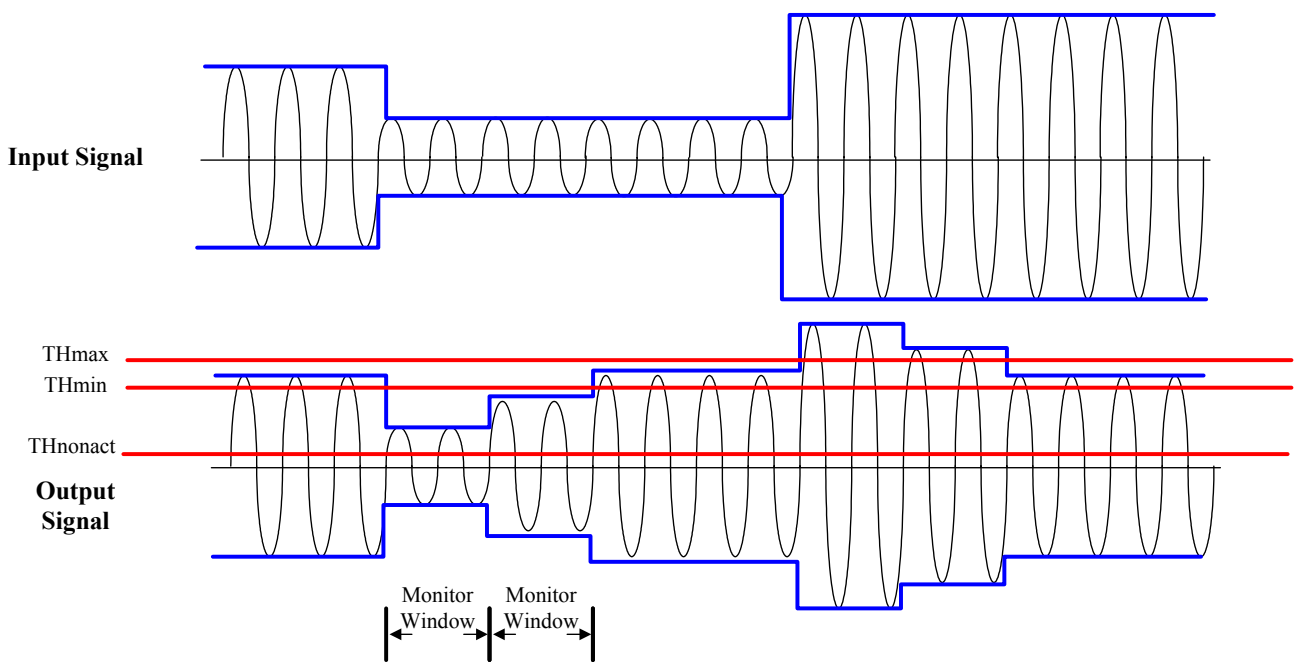
Figure 14. AVC Behavior
