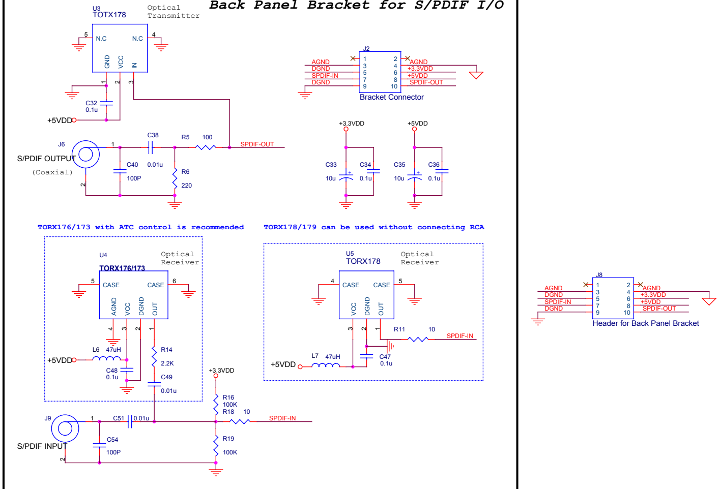
Onboard Header and Reference Back Panel Schematic for S/PDIF I/O
