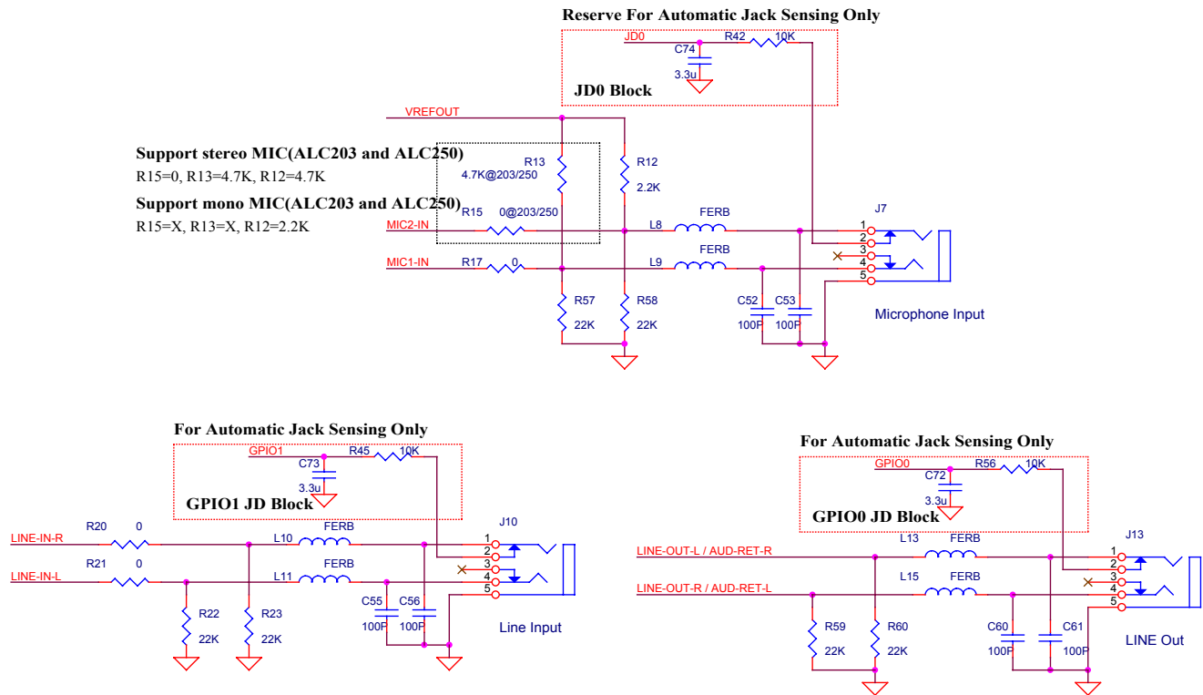
I/O Connection Schematic
