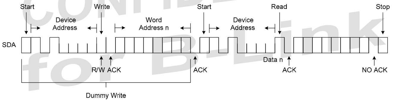
Figure 8. Random Read
