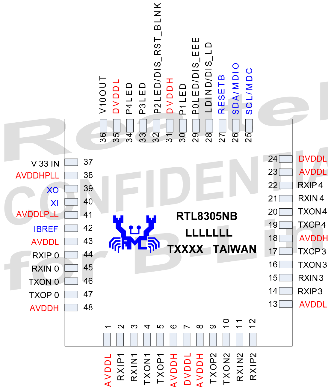
Figure 2. Pin Assignments
