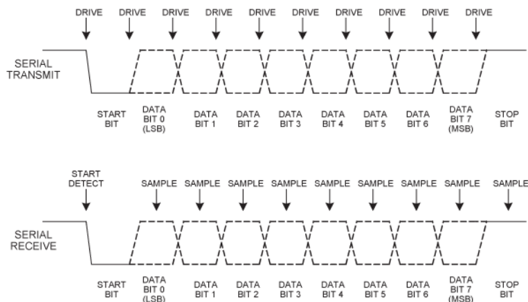
Figure 15. UART Waveform
