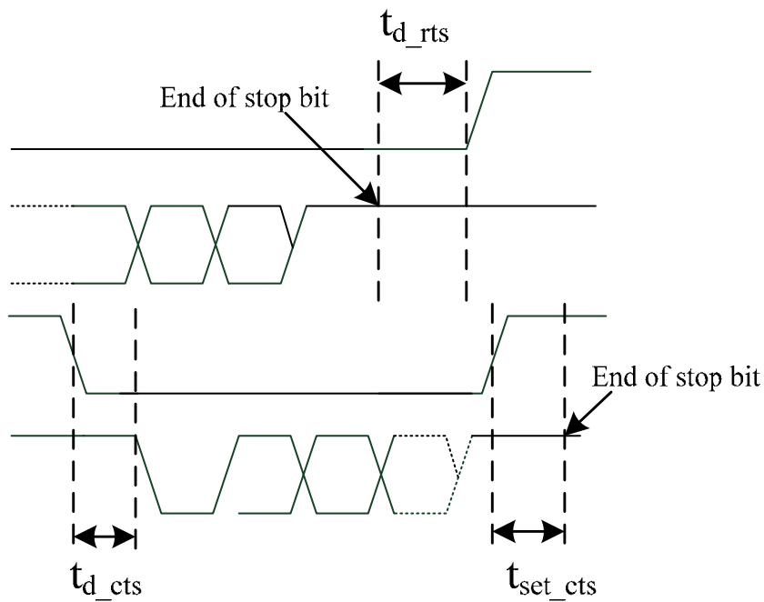
Figure 18. UART Characteristics
