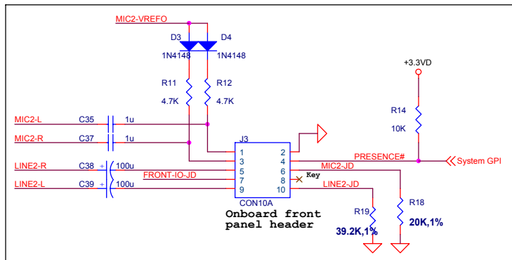
HD Audio Front Panel I/O Cable
