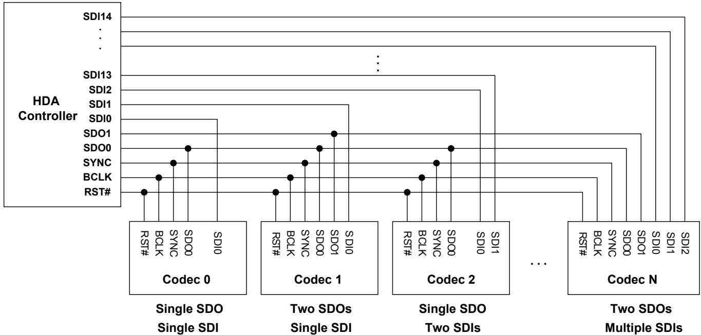
Figure 5. Signaling Topology
