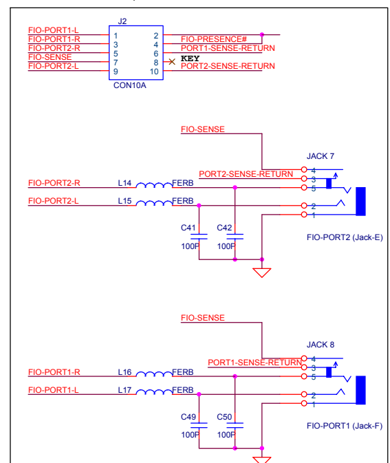
HD Audio Front Panel I/O Cable
